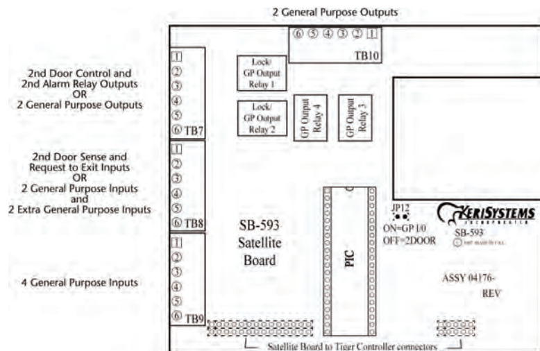
SB-593 Expansion Board
